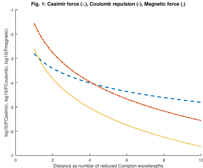
Figure 1: Trends of Casimir, Coulomb and magnetic force as a function of distance.
